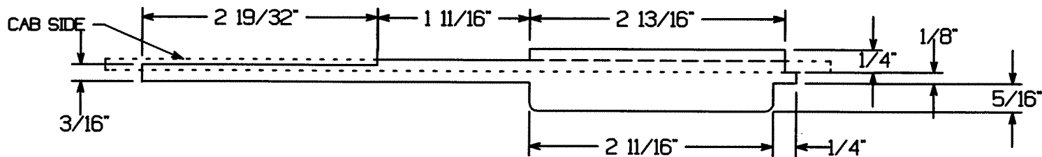
TOP VIEW OF WINDOW SILL & ARM REST MAKE FROM 1/8 ANGLE
