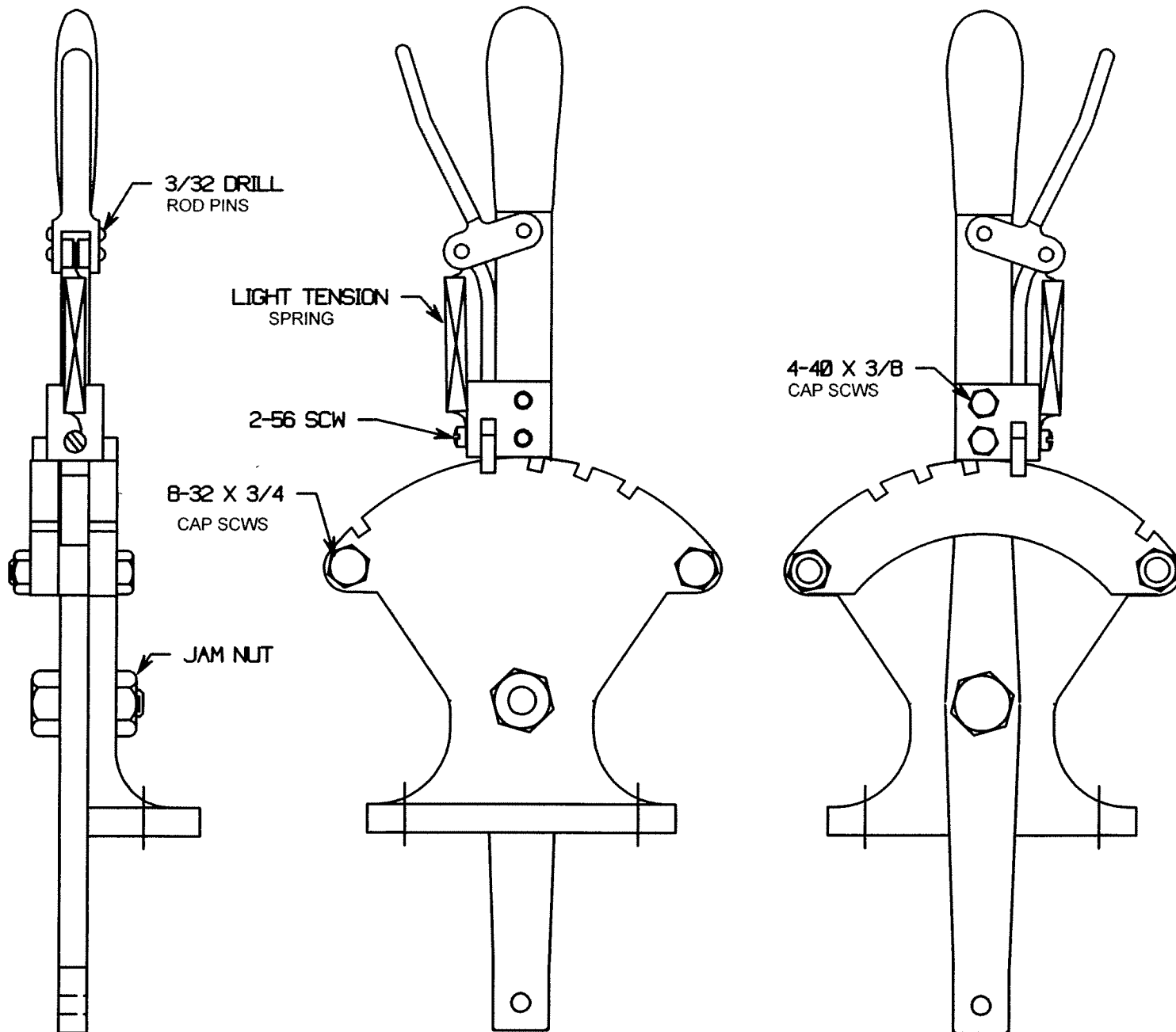
REVERSE STAND ASSY 1 1/2" LIGHT MOGUL SHEET 28a
