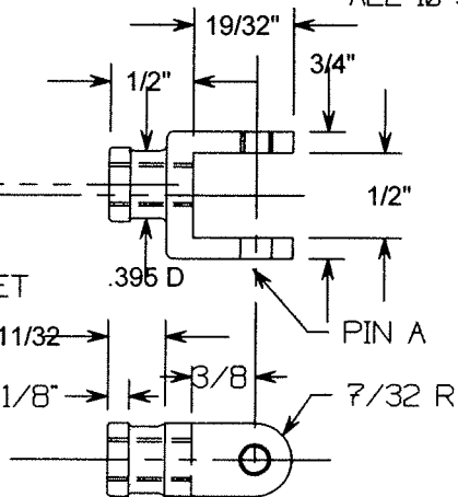
VALVE ROD FITTING CRS 2 REQD
