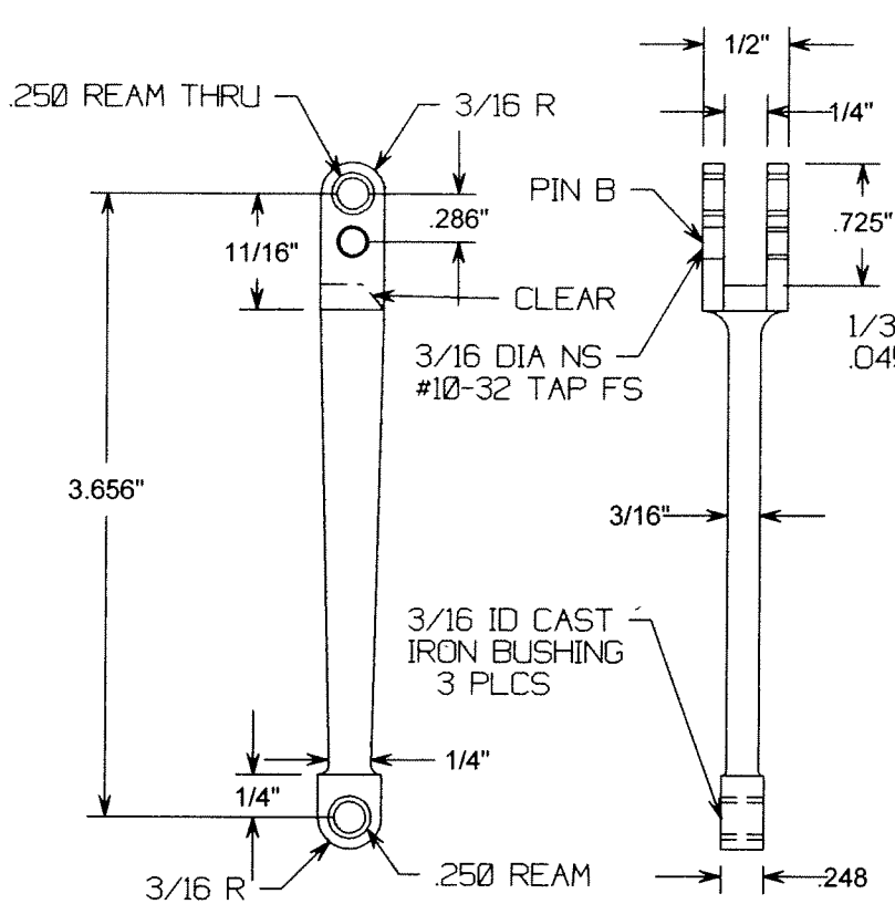
COMBINATION LEVER CRS 1 RH & 1 LH REQD RH LEVER IS SHOWN LH WILL HAVE CLEAR ANGLE ON OPOSITE SIDE
