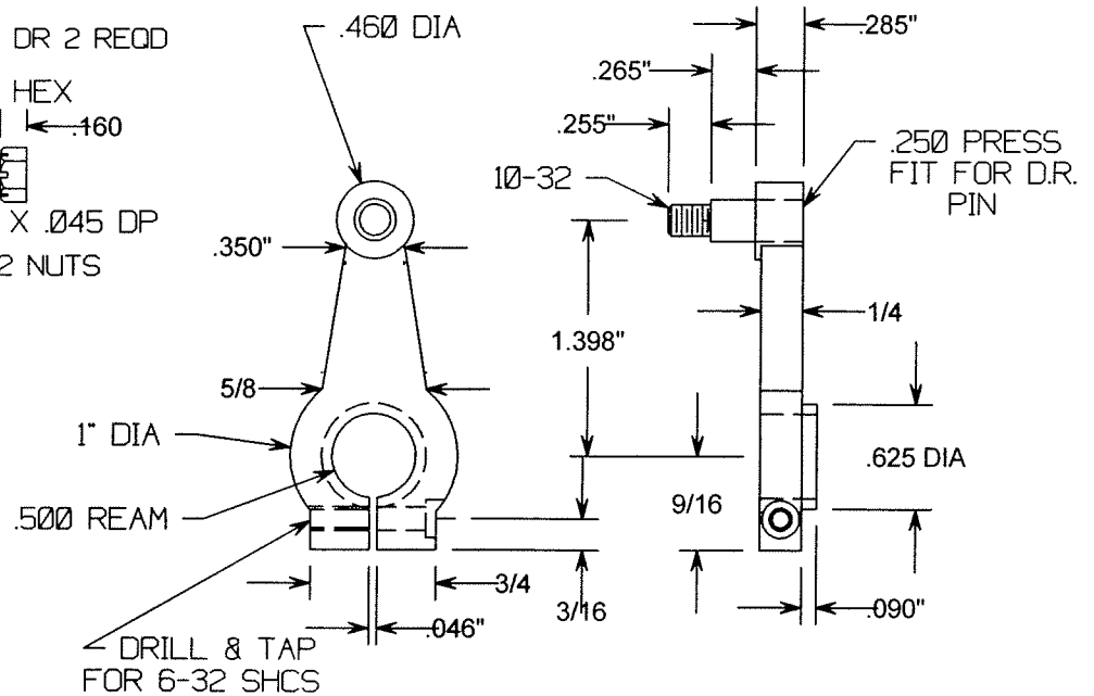
RETURN CRANK CRS 2 REQD
