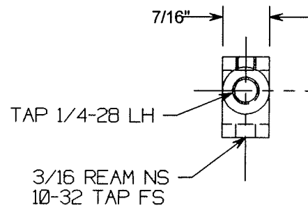
COMBINATION LEVER CRS 1 RH & 1 LH REQD RH LEVER IS SHOWN LH WILL HAVE CLEAR ANGLE ON OPOSITE SIDE
