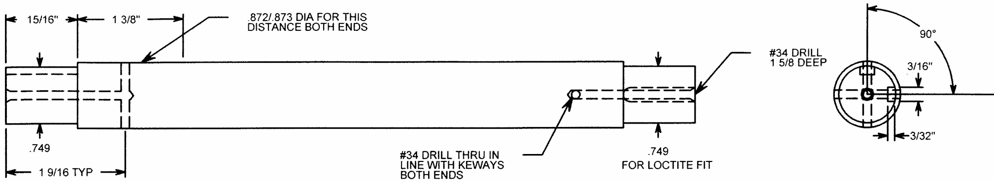
DRIVER AXLE 7/8 DRILL ROD 3 REQD
