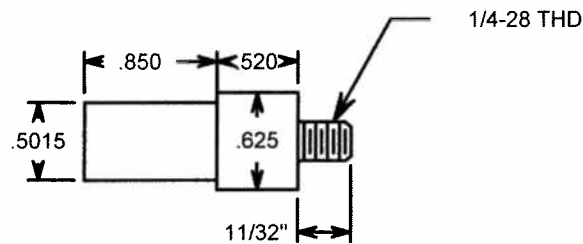
TRAILING WHEEL CRANK PIN DRILL ROD 2 REQD
