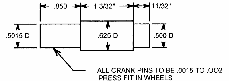
MAIN CRANK PIN DRILL ROD 2 REQD
