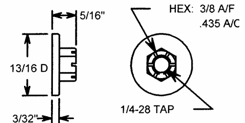
TRAILING WHEEL C. P. NUT CRS 2 REQD
