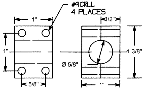
FRONT TRUCK AXLE BOX C. I. 2 REOD
