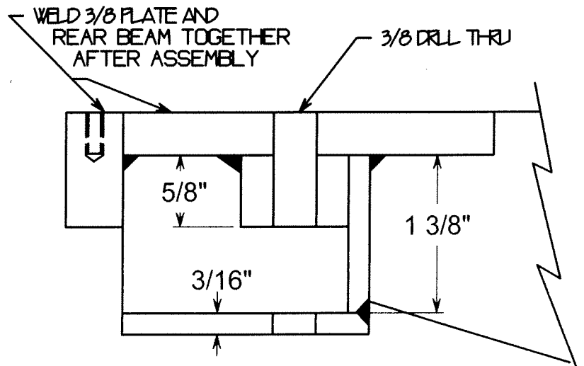
DRAW BAR POCKET CRS WELDMENT
