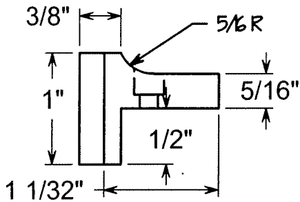
REAR FRAME BUMPER 1 REQ'D CRS
