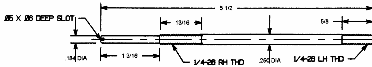
VALVE ROD SS 2 REOD
