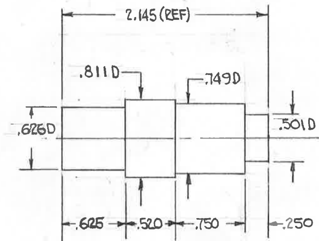
#2141 MAIN DRIVER PIN STEEL 2 REQD CASE HARDEN
