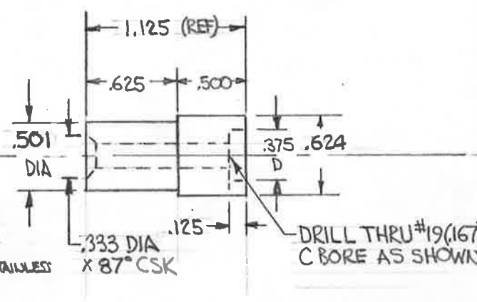
#4141 REAR CRANKPIN STEEL 2 REQD CASE HARDEN
