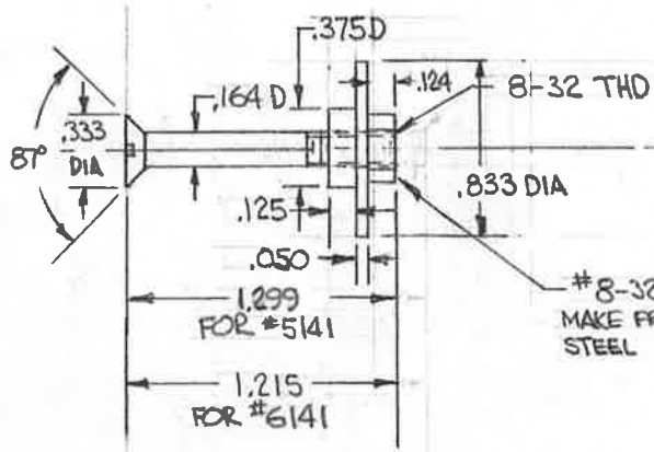
#5141 LOCK ASSY - STEEL 2 REQD FOR REAR PIN #6141 LOCK ASSY - STEEL 2 REQD FOR FWD PIN
