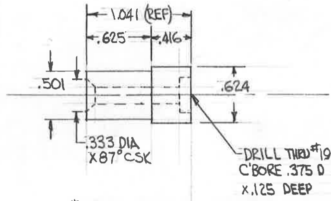
#3141 FRONT CRANK PIN STEEL 2 REQD CASE HARDEN
