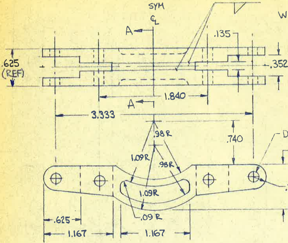
# CROSS-BAR STEEL 1 REQD ✓
