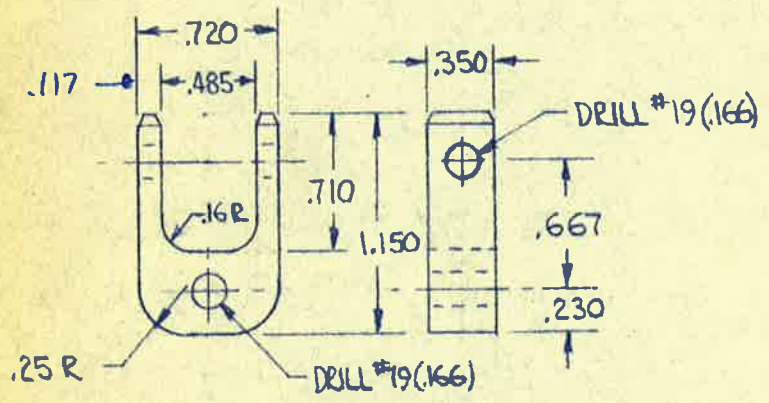
# CROSS-BAR UPPER LINK STEEL 2 REQD ✓
