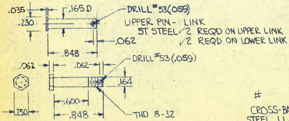
LOWER BOLT - UPPER LINK, ST STEEL 2 REQD ✓
