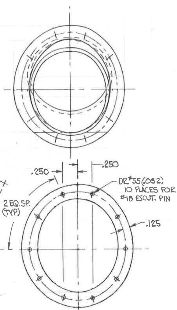
FLAT PATTERN ATTACH RING
