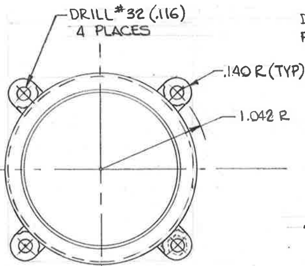
TOP VIEW OF STACK ONLY
