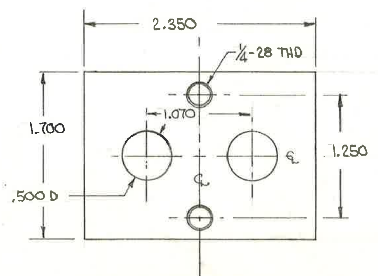
NOZZLE FACE AS SEEN AT SECTION A-A
