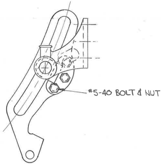
FINAL ASSY
