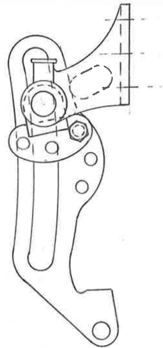
INSTALLING FIRST BOLT
