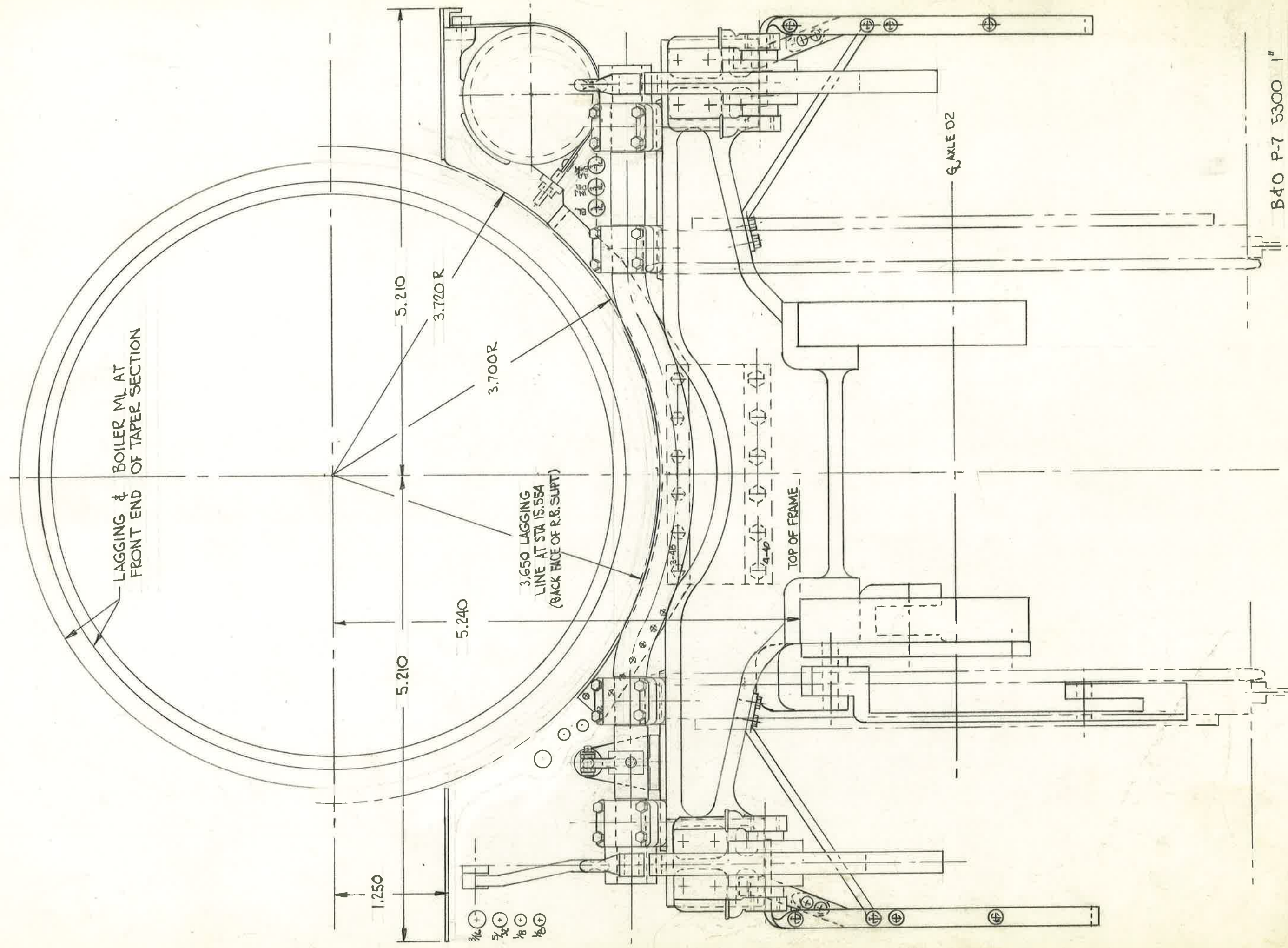
SECTION LOOKING AFT AT MOTION BEAM
