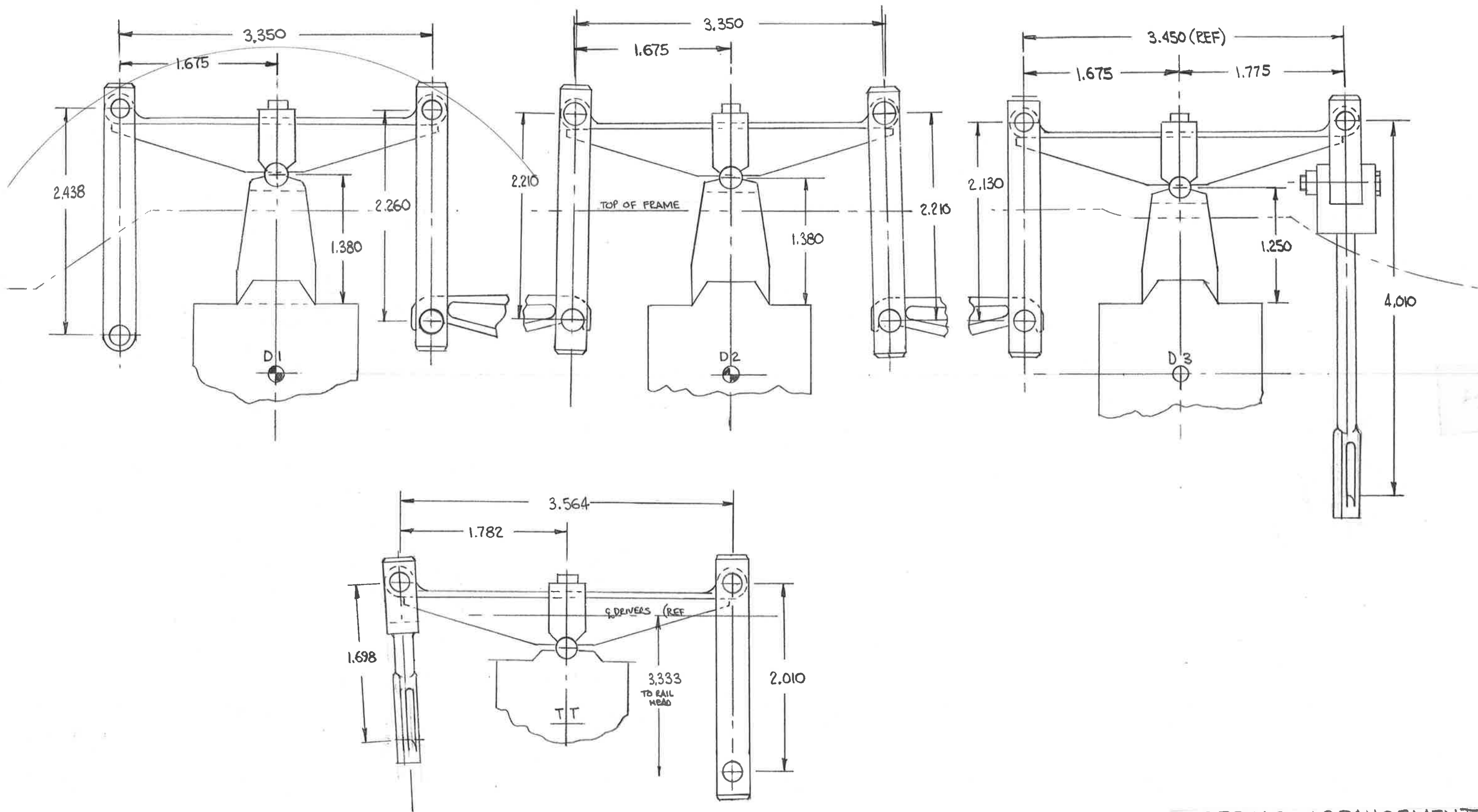
SPRING ARRANGEMENT 1" B&O P-7 I.D. ALKIRE 1961
