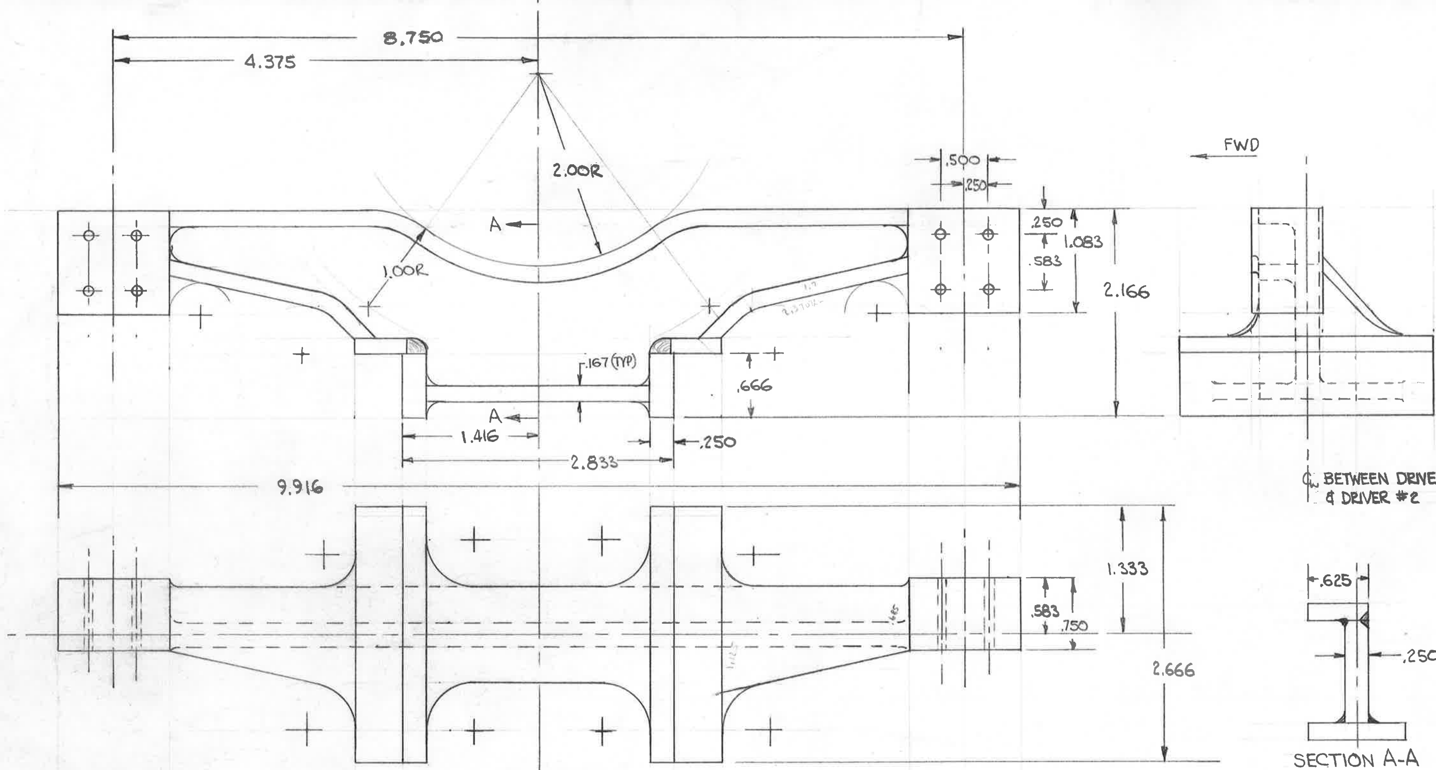
MOTION BEAM 1"=1' B&O P-7
