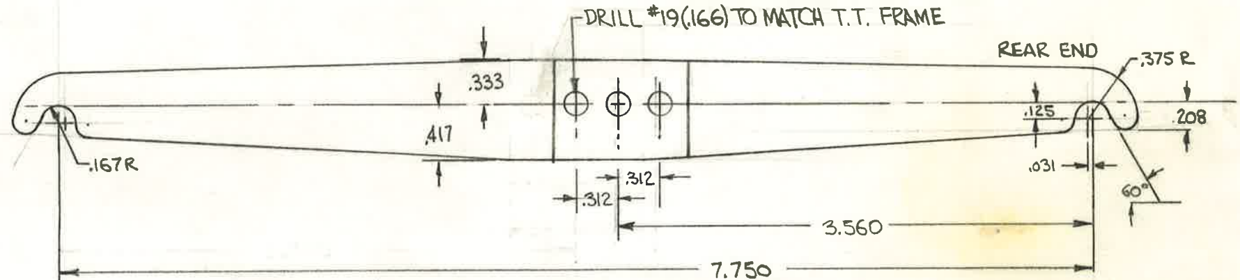
#6145A TRAILER TRUCK EQUALIZER STEEL 2 REQD FOR USE WITH LITTLE ENGINES T.T. CASTING .250 THICK AT CENTER .190 AT ENDS UNIFORM TAPER
