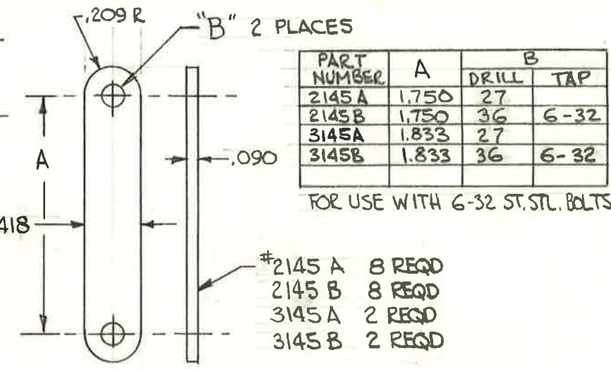
LINK STEEL SEE CHART FOR REQS.
