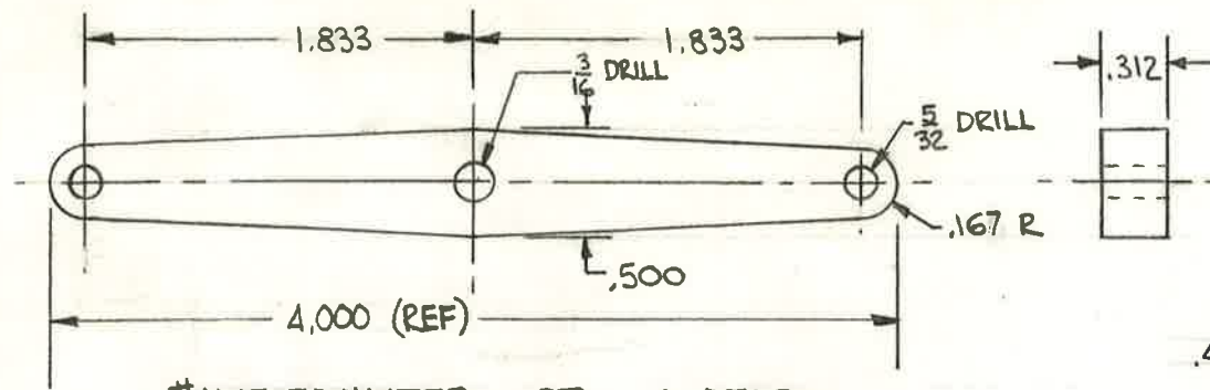
#1145 EQUALIZER STL. 4 REQD
