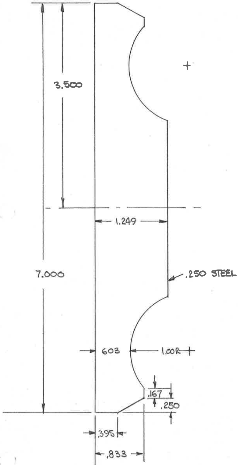
VERTICAL BEAM CRADLE REAR BUMPER B&O PAC PRES 1" I.D. ALKIRE 1961
