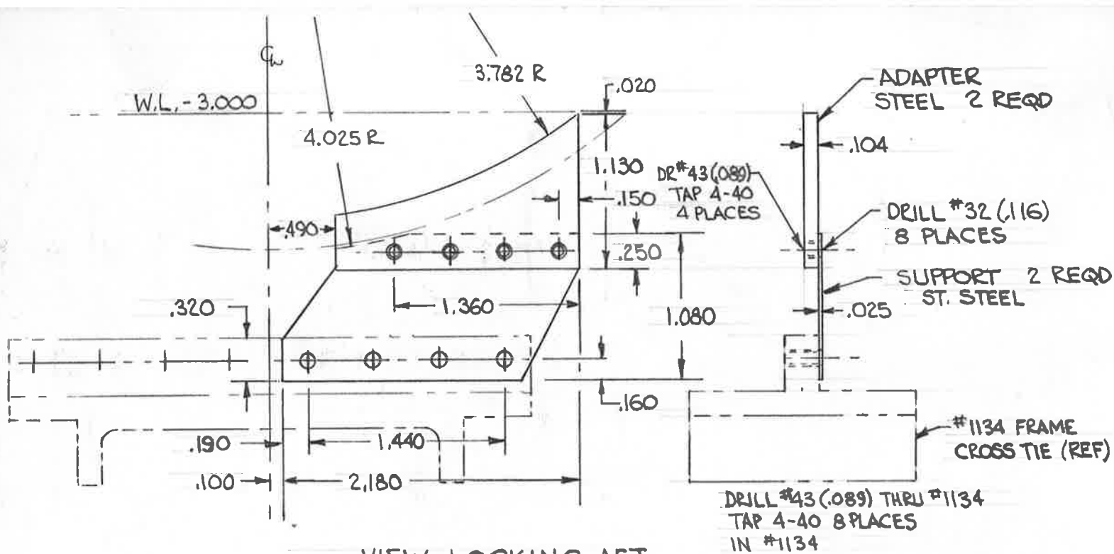
VIEW LOOKING AFT BOILER SUPPORT AT FRAME CROSS-TIE
