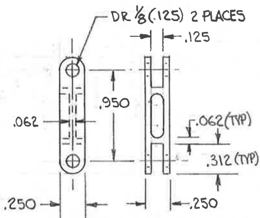
THROTTLE LEVER LINK STEEL 1 REQD
