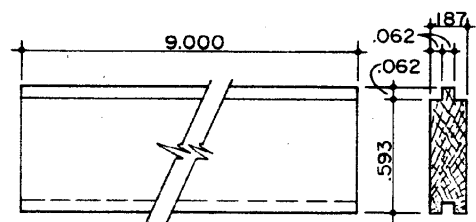
342 TENDER DECKING Seasoned Oak 70 Required
