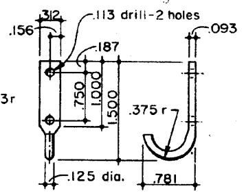
246 RERAILER HOOK Cold Rolled Steel 4 Required
