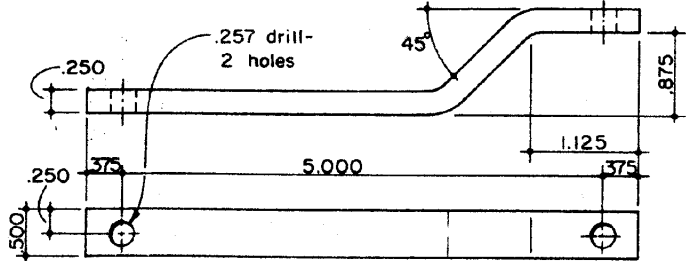
290 TENDER DRAWBAR Cold Rolled Steel 1 Required
