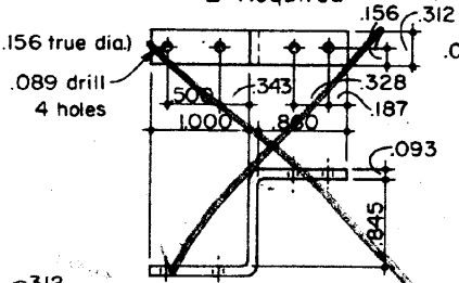
253 FRONT STEP BRACE Cold Rolled Steel 2 Required
