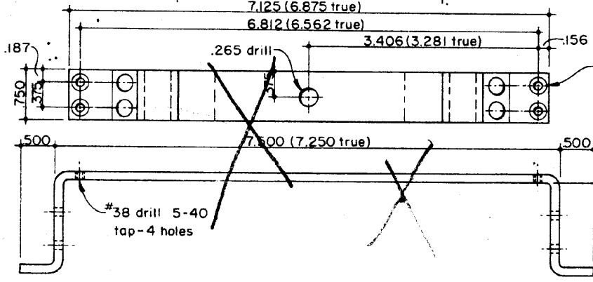
247 BODY BOLSTER Cold Rolled Steel 2 Required
