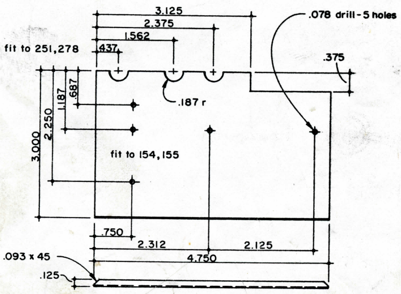
279 PILOT BEAM APRON .018 Cold Rolled Steel 2 Required: (1 as shown - 1 opposite)
