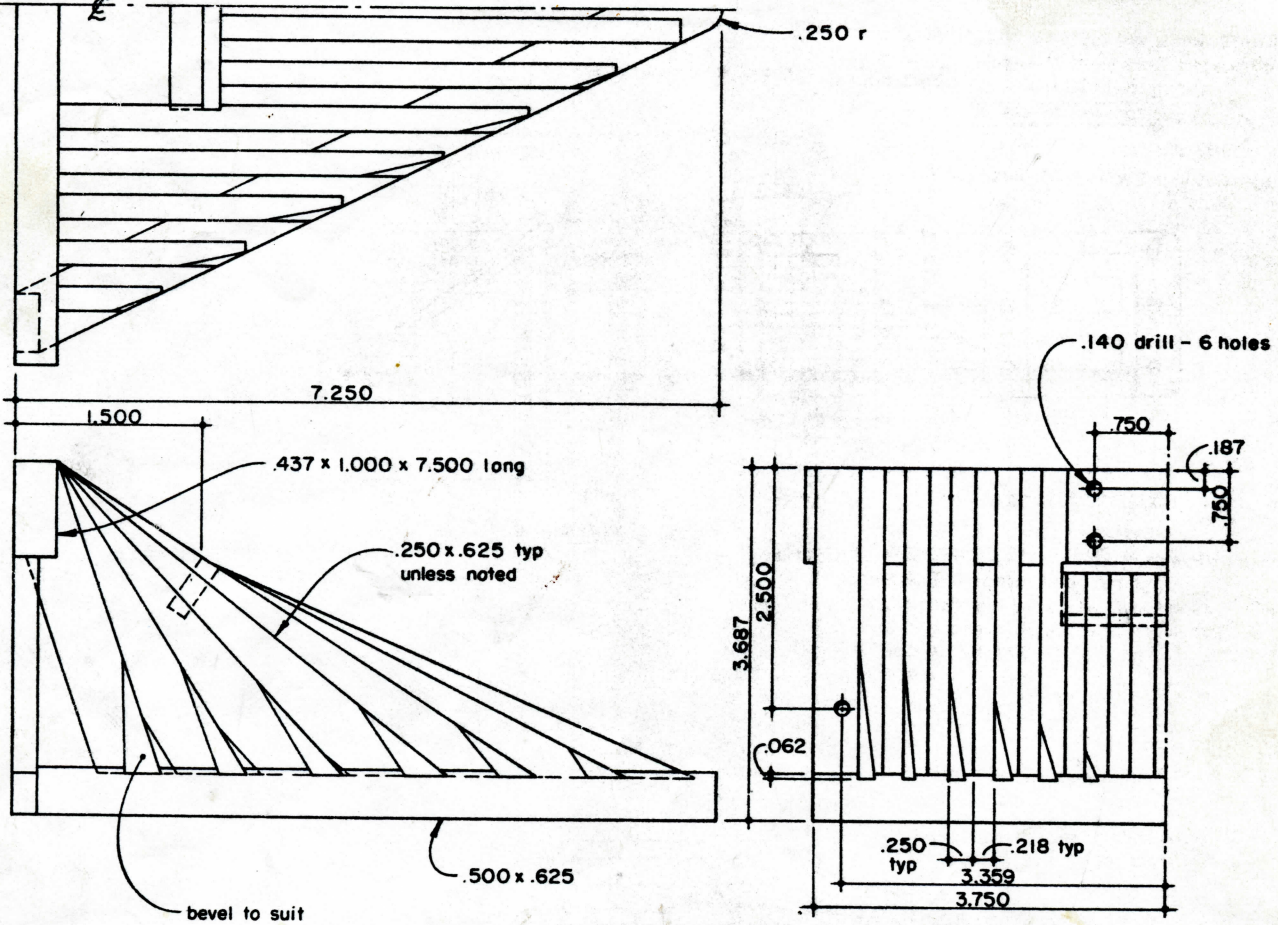
369 WOOD PILOT Hardwood 1 Required
