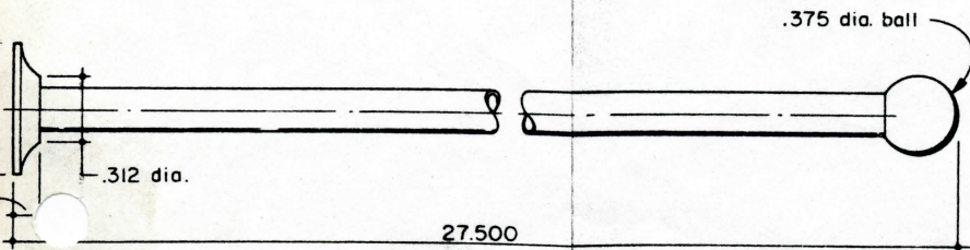
382 HANDRAIL .187 O.D. Tubing 2 Required
