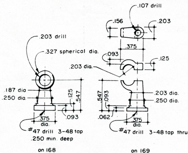
314 SHORT HANDRAIL STANCHION Brass 2 Required
