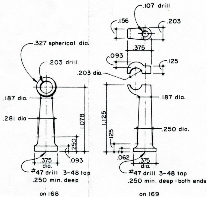
316 LONG HANDRAIL STANCHION Brass 2 Required
