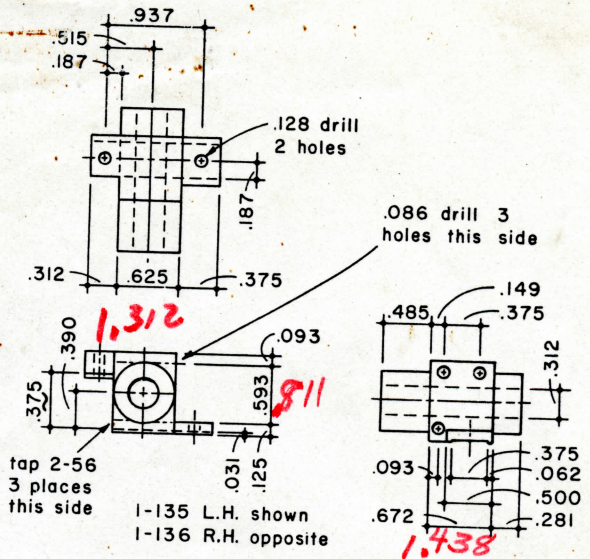
135, 136 ROCKER BEARING Brass 2 Required
