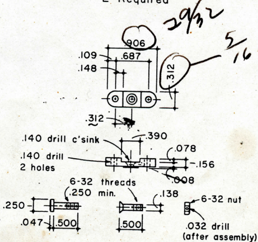
153 LINK SADDLE Cold Rolled Steel 2 Required
