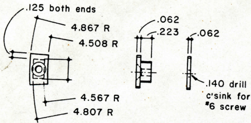
175 LINK BLOCK Cold Rolled Steel 2 Required
