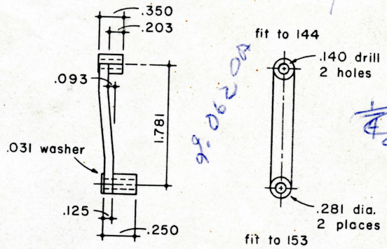
135, 136 ROCKER BEARING Brass 2 Required
