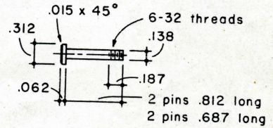
204 VALVE LINK HANGER Cold Rolled Steel 2 Required
