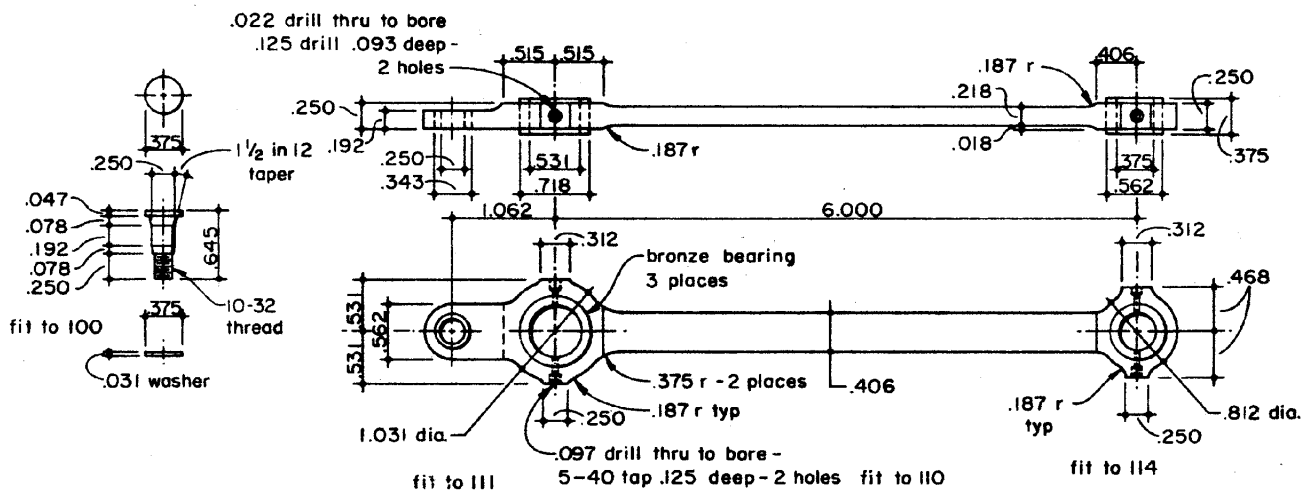
211/212 FRONT ROD Cold Rolled Steel 2 Required: (1 as shown, 1 opposite)
