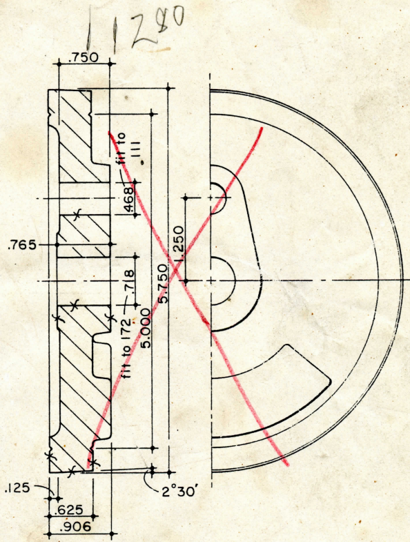
127 MAIN DRIVER Gray Iron Casting 2 Required
