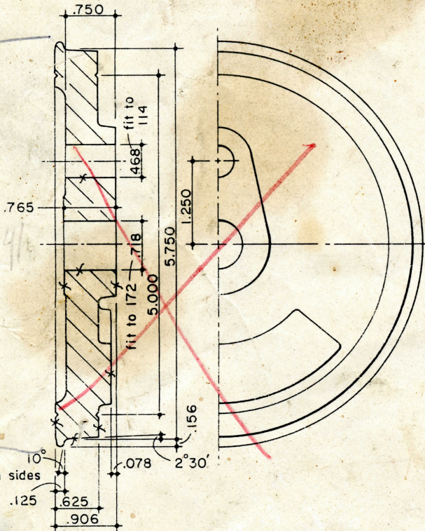
129 FRONT & REAR DRIVER Gray Iron Casting 4 Required
