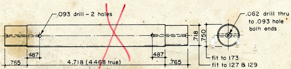
6.248 172 AXLE Cold Drawn Steel 3 Required
