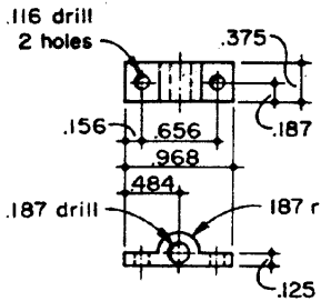
115 SHAKER SHAFT BEARING Cold Rolled Steel 2 Required
