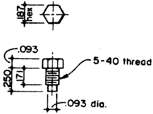
110 BEARING STOP SCREW Cold Drawn Steel 8 Required
