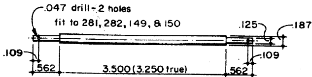
282 DRIFTER CROSSOVER SHAFT Cold Rolled Steel 1 Required
