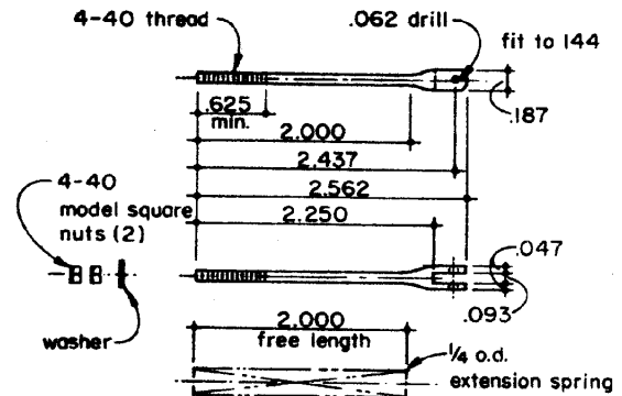
376 SPRING GUIDE Cold Drawn Steel 1 Required
