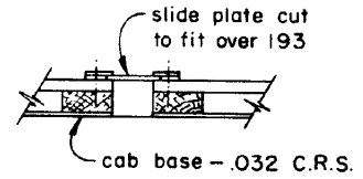
section thru floor at Johnson bar
